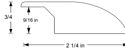
9/16" OVERLAP REDUCER
