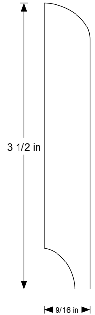
BASEBOARD
