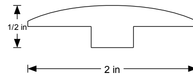
3/8" T-MOLDING
