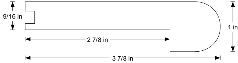
9/16" STAIRNOSE
