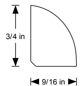
BASE SHOE
