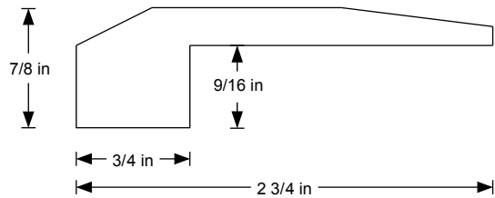
9/16" THRESHOLD
