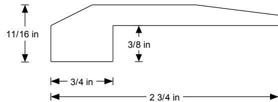
3/8" THRESHOLD
