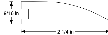
9/16" Flush REDUCER
