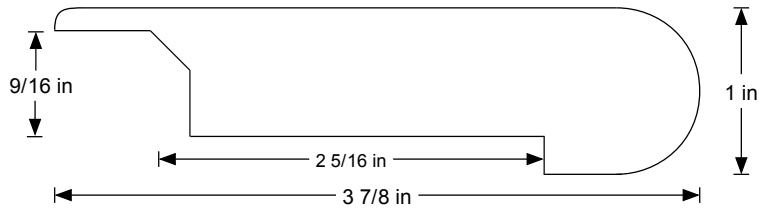
9/16" OVERLAP STAIRNOSE
