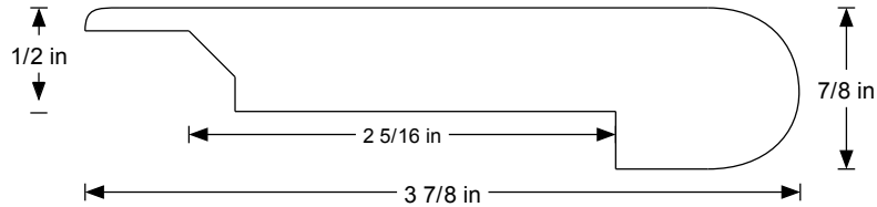
3/8" OVERLAP STAIRNOSE
