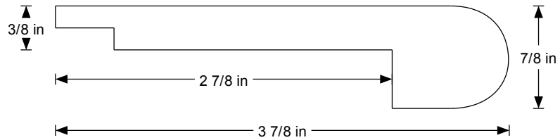
3/8" Drop n Lock Flush STAIRNOSE
