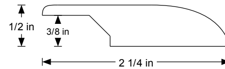
3/8" OVERLAP REDUCER
