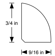
BASE SHOE
