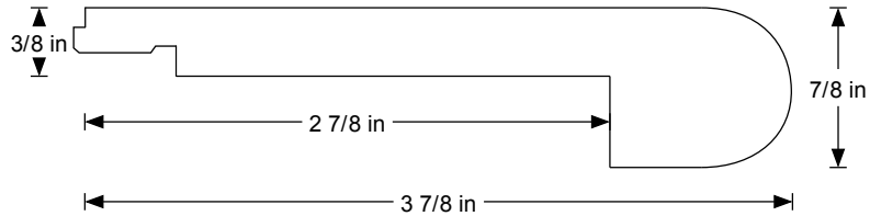
3/8" Drop n Lock G2+ Flush STAIRNOSE
