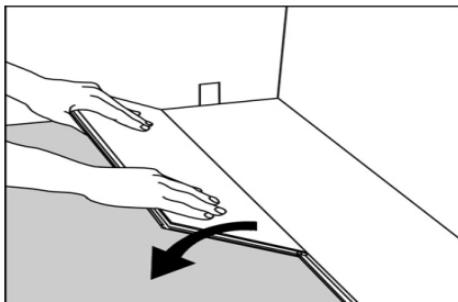
Fig 7. Place the floor board an angle against the floorboard in the previous row, press forward and fold down at the same time.
