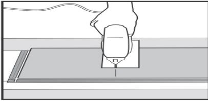
Fig 5. Second row. First plank min length 3/8" to 1/2". Put a distance against the wall.
