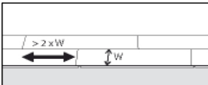
Fig 7. Place the floor board an angle against the floorboard in the previous row, press forward and fold down at the same time.
